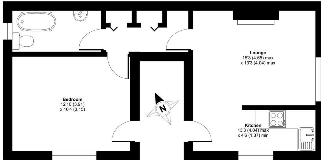
GROUND FLOOR
